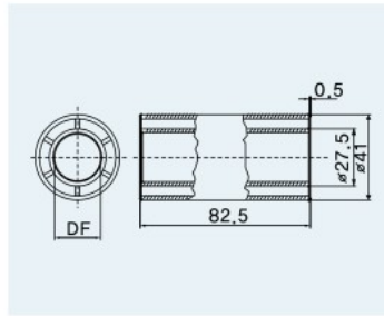
CHAIN STRETCHER ROLLER
