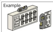
For mounting of distribution panel board embedded power outlet
