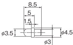
PB107形
