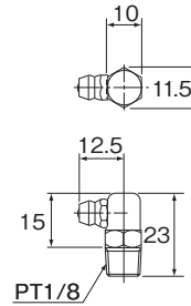
C-PT1/8形
