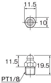
A-PT1/8形
