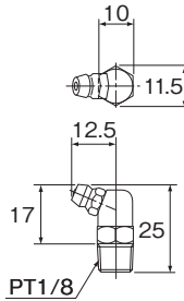
B-PT1/8形
