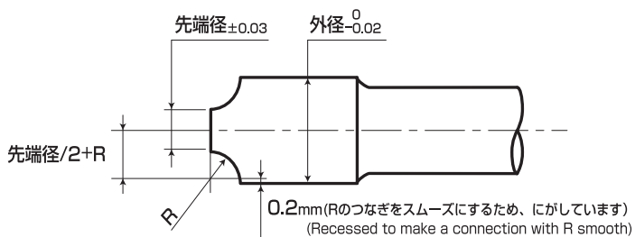
<FA GCCRCL 詳細形状図 Detailed drawing of FA GCCRCL>
