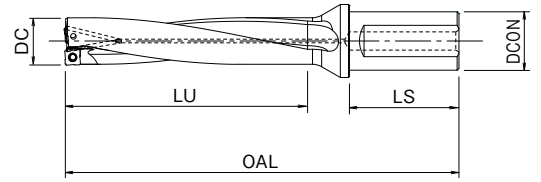
油穴付き with Coolant Hole
