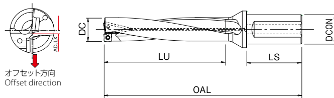
油穴付き with Coolant Hole
