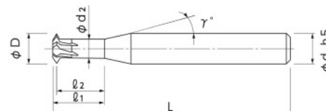
6-Flute
