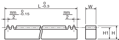
Gear-Cutting Reference Surface
