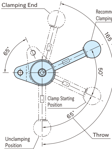
Counterclockwise Clamping
