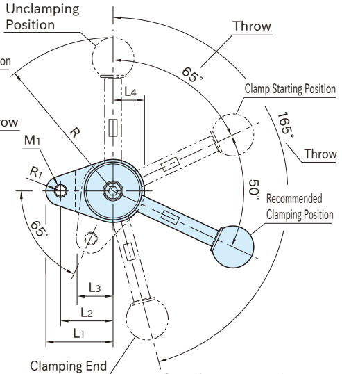
Clockwise Clamping
