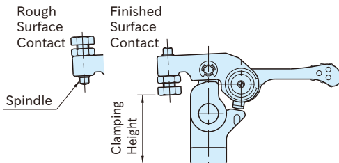
Clamping Position
