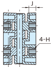
EMH-SS (Tapped)
