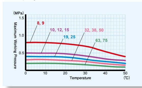
E-KYS: KY SUNFOODS HOSE
