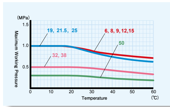
E-STB: Oil-Proof PRESSURE HOSE
