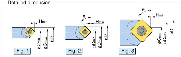
Detailed dimension
